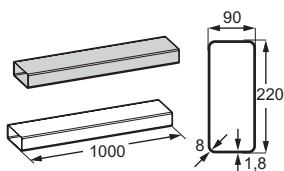
K1 Half pipe kit
