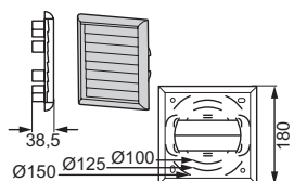
S10 M2CKCF12U External grid with gravity flaps
