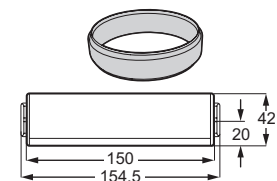
S6 M2CKCF08U Female round connection (ø150mm)
