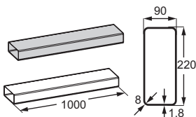
S2 M2CKCF05U Rectangular pipe, 1m (220x90mm)
