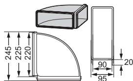
S4 M2CKCF04U Rectangular Horizontal 90° curve (220x90mm)
