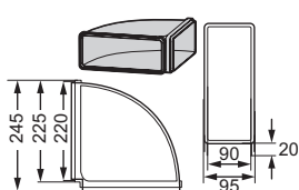
K4 Rectangular Horizontal 90°, curve (220x90mm)
