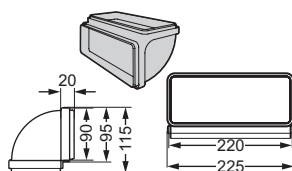
K2 Rectangular vertical 90° curve
