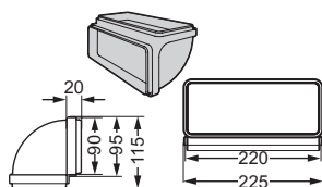
S7 M2CKCF09U Rectangular Vertical 90° curve (220x90mm)
