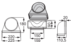
S1 M2CKCF03U Vertical 90° curve from rectangular (220x90mm) to round (ø150mm)
