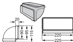
K2 Rectangular Vertical 90°, curve (220x90mm)
