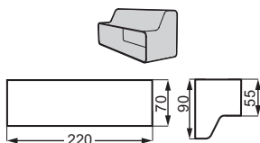
S9 M2CKCF11U Rectangular straight reduction (220mm) from 90 to 55 mm
