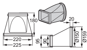
S3 M2CKCF02U Straight connection from rectangular (220x90mm) to round (ø150mm)
