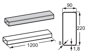
K3 Rectangular pipe, 1,2m (220x90mm)
