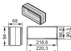
K5 Connector
