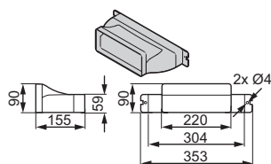
K6 Diffuser
