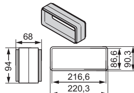
S12 M2CKCF06U Connector
