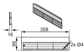
K7 Grid
