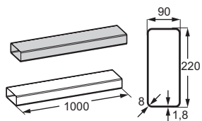
K1 Rectangular pipe
