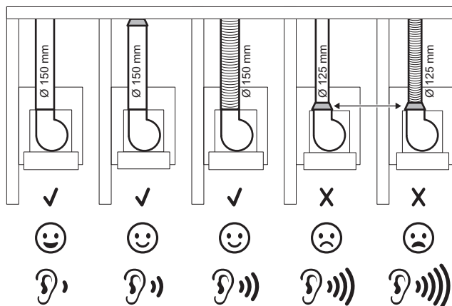
Motor outlet diameter 150 mm
